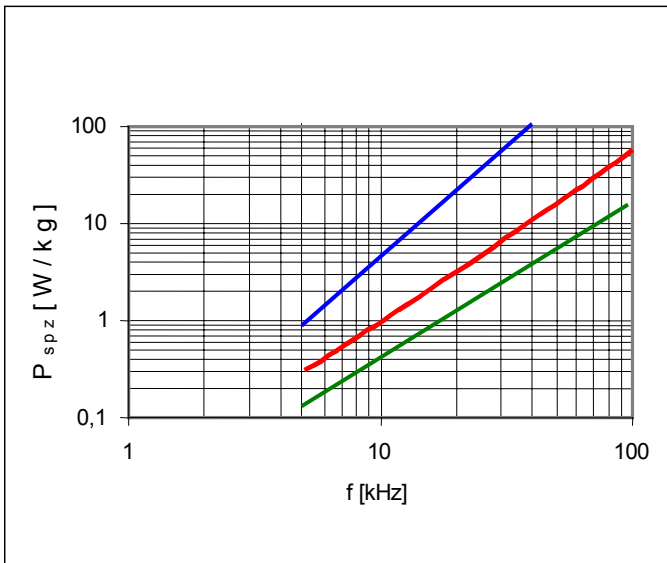
Losses ( — B = 0,15\text{T} , — B = 0,3\text{T} , — B = 0,6\text{T} )
