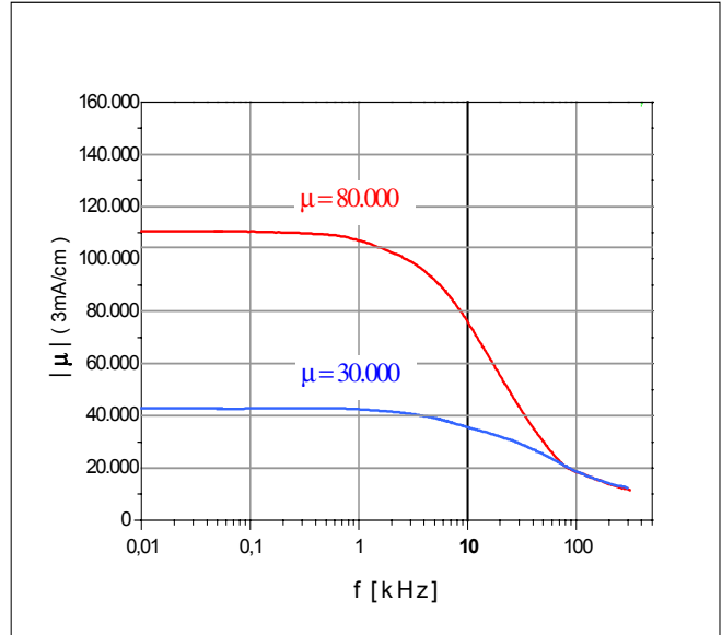
Frequency response
