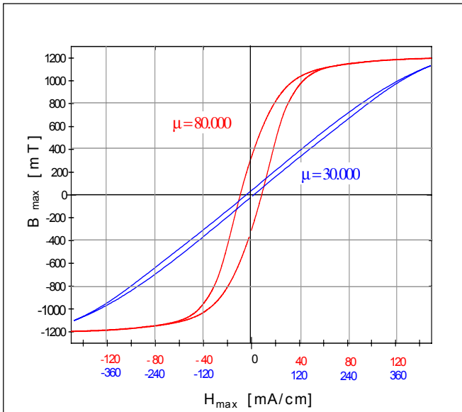
Possible hysteresis shapes (static, 50 Hz)
