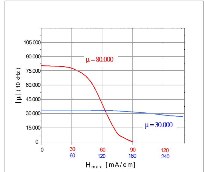
DC-behaviour
